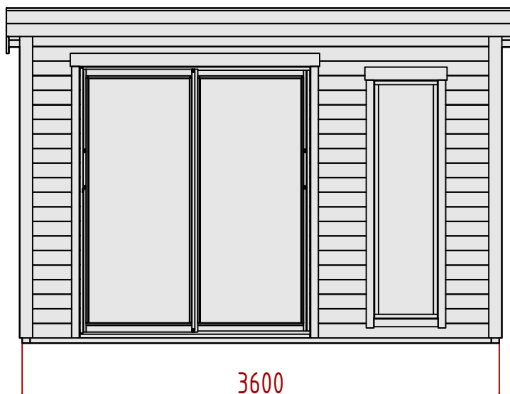
FRONT FASADE
